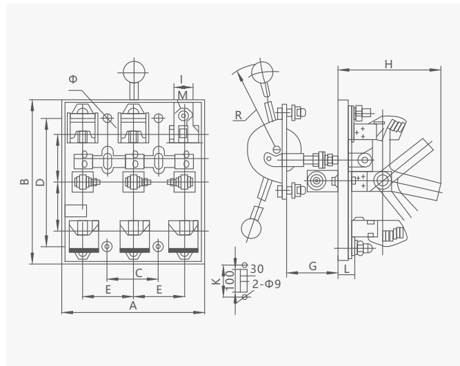
HS13-600~1500、HS13B-600~1500接线图(尺寸见G表)
